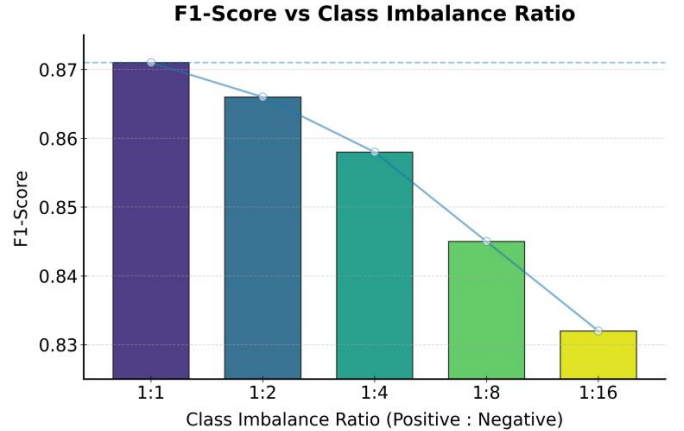
Figure 5. Sensitivity experiment of F1-Score to class imbalance
