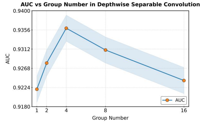
Figure 3. Sensitivity experiment of the number of channel groups of depthwise separable convolution on AUC
