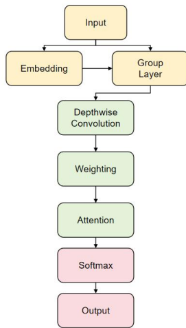
Figure 1. Overall model architecture
