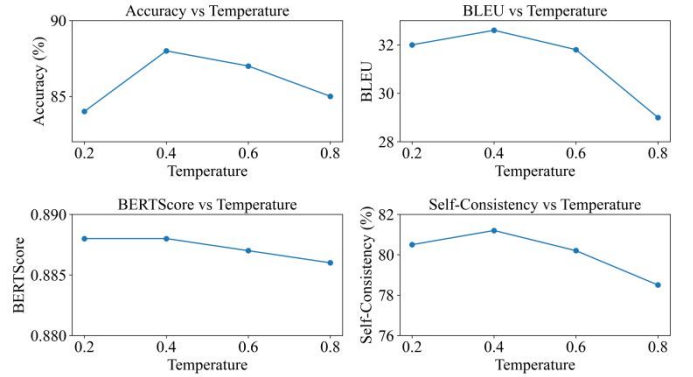
Figure 3. The effect of different inference temperature settings on experimental results
